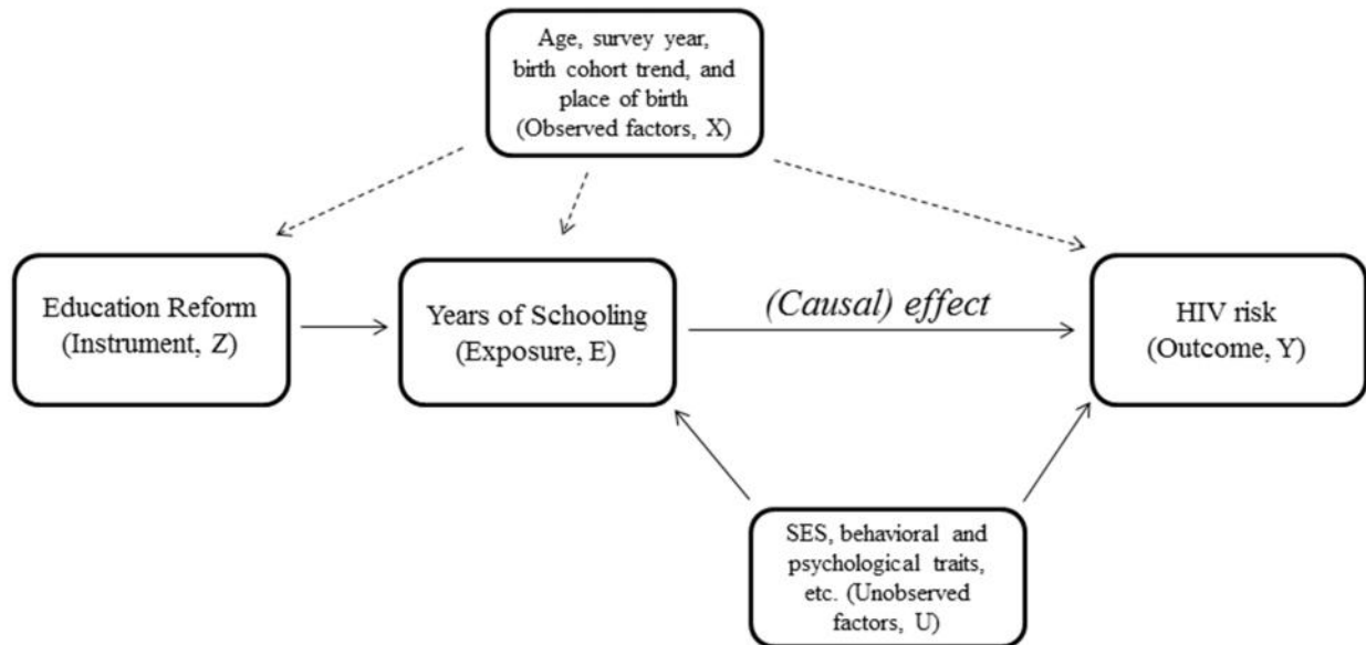
Figure 1: Causal Diagram.
